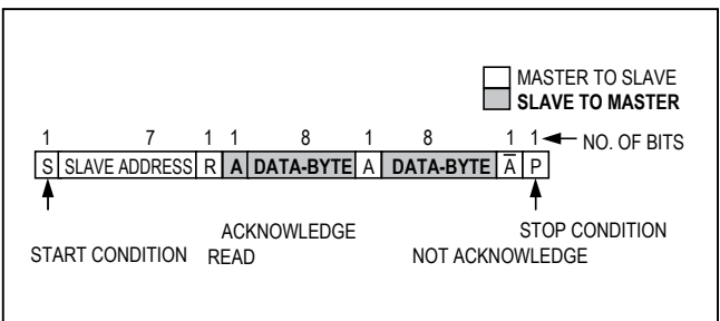
Figure 7. Read Cycle
