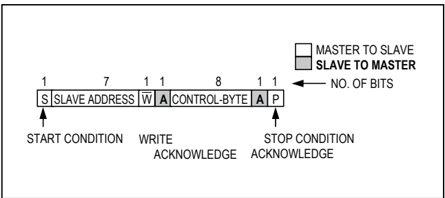
Figure 6. Write Cycle
