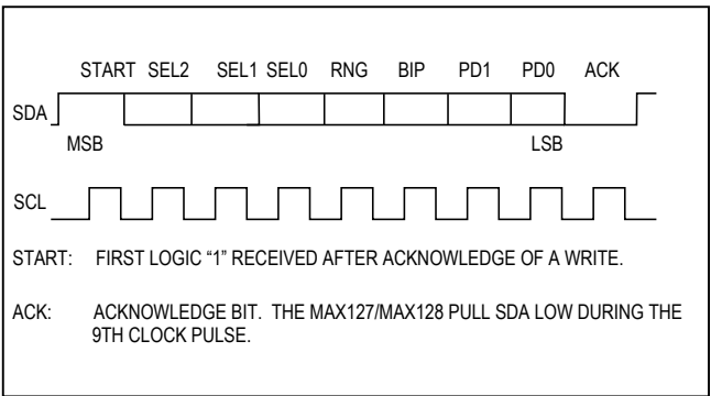
Figure 8. Command Byte
