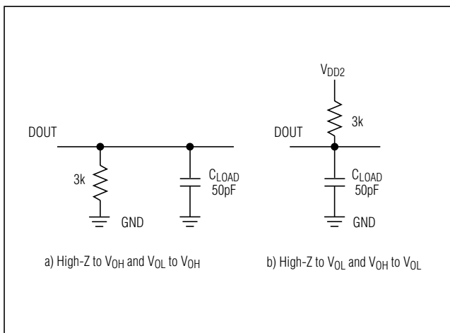
Figure 1. Load Circuits for Enable Time
