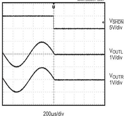
ENTERING SHUTDOWN TRANSIENT MAX13330/31 toc27
