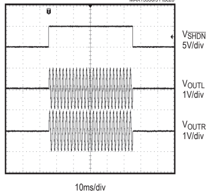
POWER-UP/-DOWN TRANSIENT MAX13330/31 toc28
