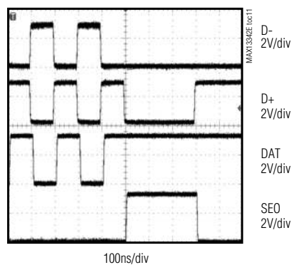
MAX13342E/MAX13345E RECEIVING
