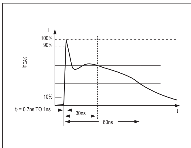
Figure 1d. IEC 61000-4-2 ESD Generator Current Waveform
