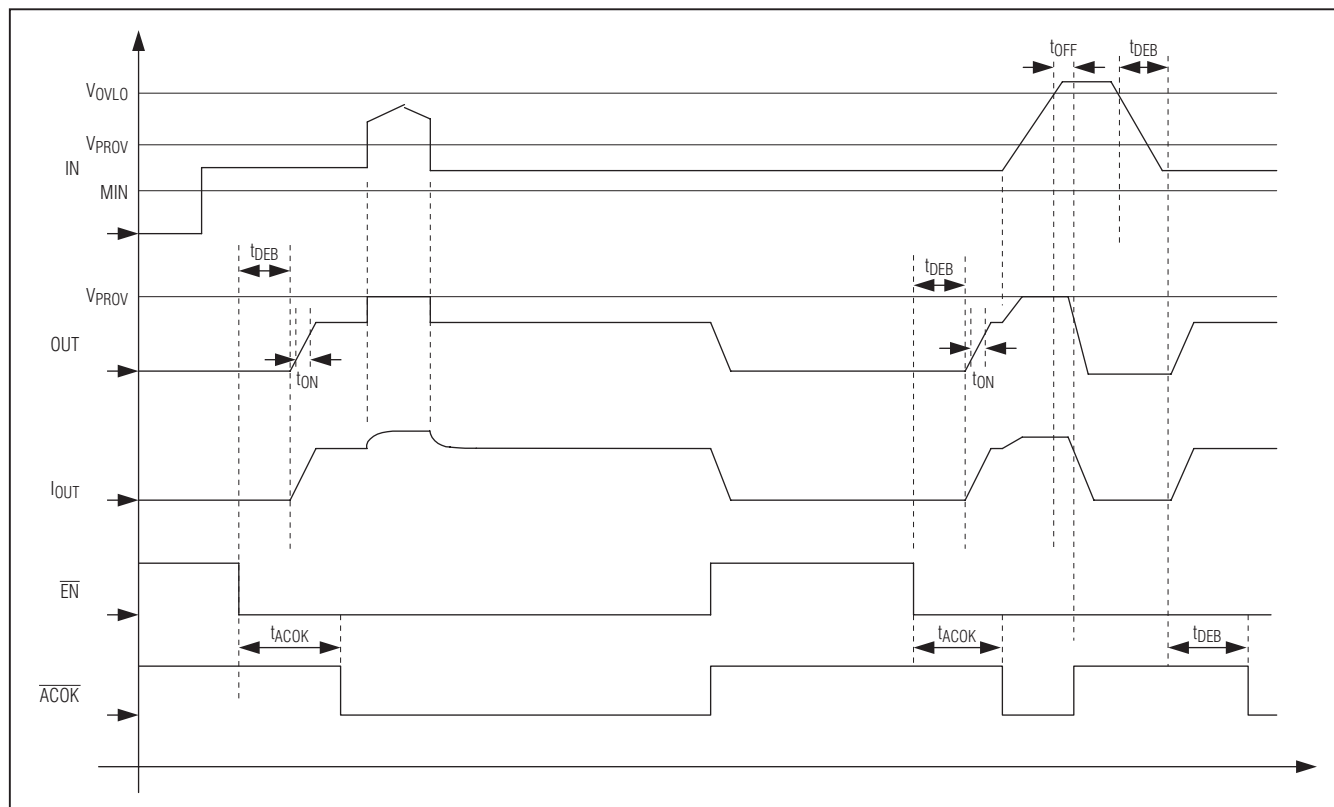
Figure 1. Enable/Select Time
