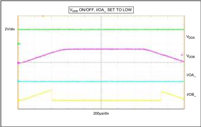
Figure 8. Undervoltage-Lockout Behavior (I/OA_ Set Low)
