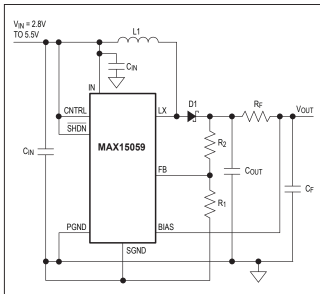
Figure 2. Typical Operating Circuit with RC Filter
