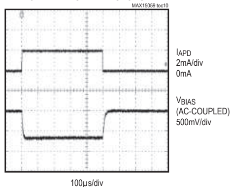
LOAD-TRANSIENT RESPONSE
