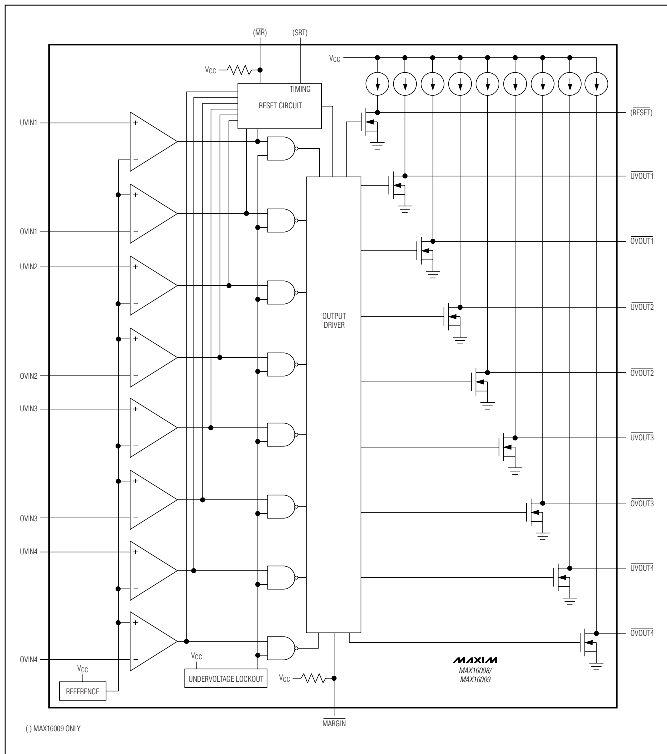
Figure 1. Functional Diagram
