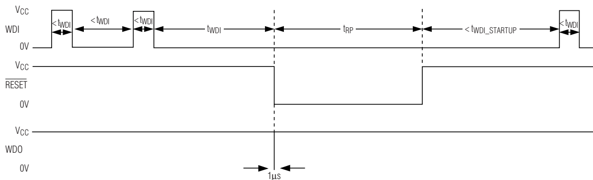
Figure 8. Watchdog Startup Sequence with Watchdog \overline{\text{RESET}} Enable Bit (r55h[7]) Set to '1'
