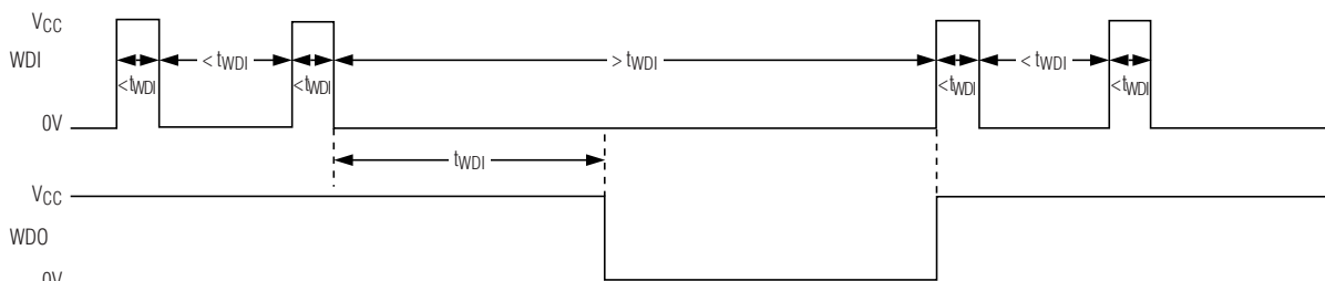
Figure 7. Watchdog Timer Operation
