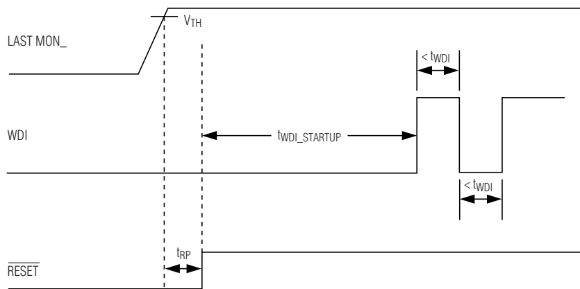
Figure 6. Normal Watchdog Startup Sequence
