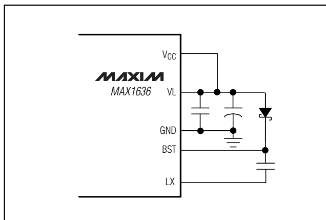
Figure 7. Capacitor Placement
