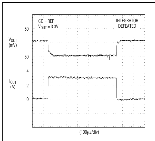
Figure 5b. Load-Transient Response with Integrator Defeated
