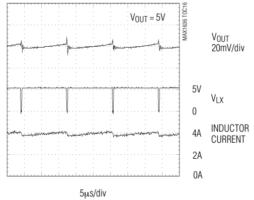
OVERVOLTAGE-PROTECTION WAVEFORMS ( V_{IN} SHORTED TO V_{OUT} THROUGH a 0.5\Omega RESISTOR)
