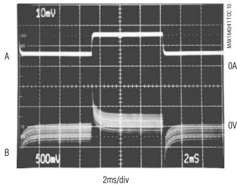
CURRENT-MODE CHANGE RESPONSE TIME
