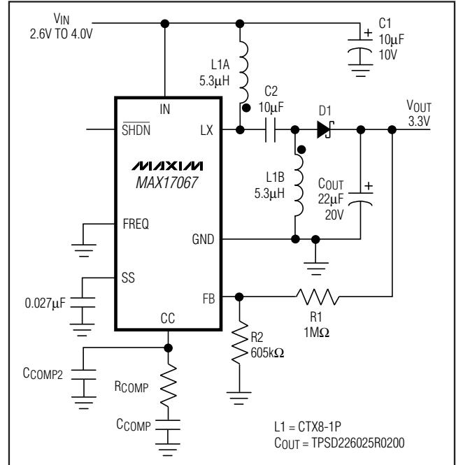
Figure 3. MAX17067 in a SEPIC Configuration
