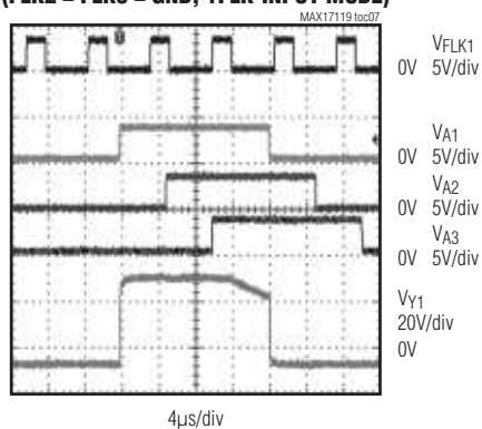
SCAN-DRIVER OUTPUT WITH GPM (FLK2 = FLK3 = GND, 1FLK-INPUT MODE)
