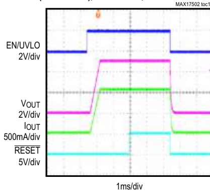
SOFT-START/SHUTDOWN FROM EN/UVLO (MAX17502F), 5V OUTPUT, FIGURE 8 CIRCUIT
