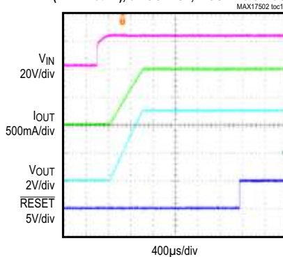
FULL-LOAD SOFT-START FROM V_{IN} (MAX17502F), 5V OUTPUT, FIGURE 8 CIRCUIT
