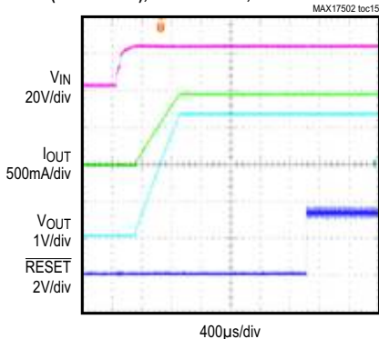
FULL-LOAD SOFT-START FROM V_{IN} (MAX17502E), 3.3V OUTPUT, FIGURE 7 CIRCUIT
