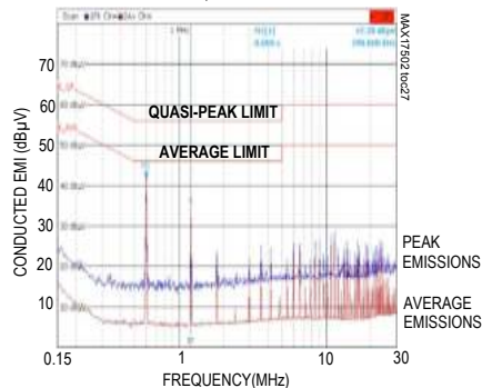
5V OUTPUT, 1A LOAD CURRENT, FIGURE 8 CIRCUIT, CONDUCTED EMI CURVE
