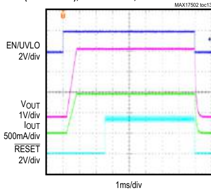
SOFT-START/SHUTDOWN FROM EN/UVLO (MAX17502E), 3.3V OUTPUT, FIGURE 7 CIRCUIT
