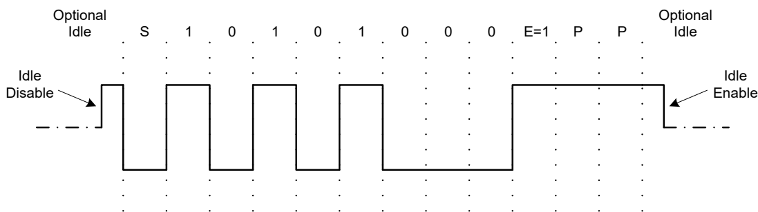
Figure 28. Preamble Character
