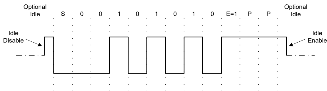
Figure 30. Stop Character
