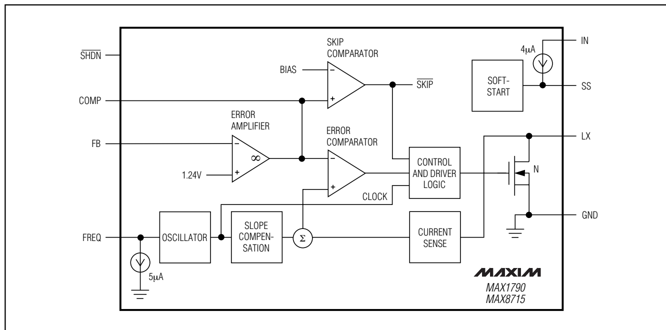
Figure 2. Functional Diagram
