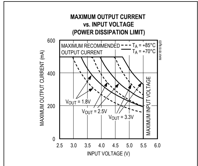
Figure 3. Power Operating Regions: Maximum Output vs. Supply Voltage
