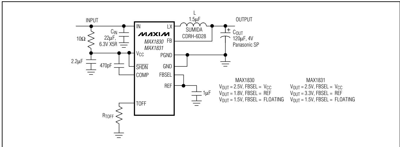
Figure 1. Typical Circuit
