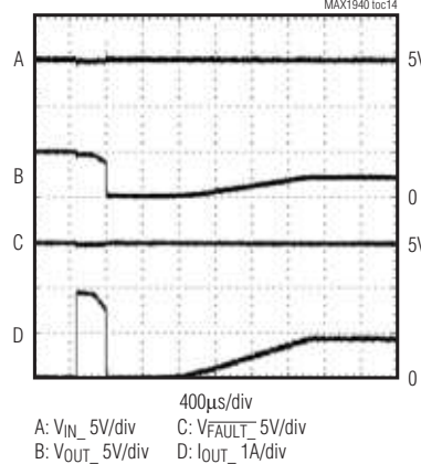
OVERLOAD RESPONSE INTO 2.5Ω (EXPANDED TIME SCALE)
