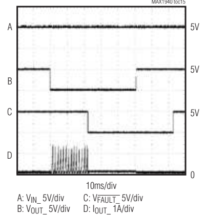
SHORT-CIRCUIT RESPONSE INTO 0Ω
