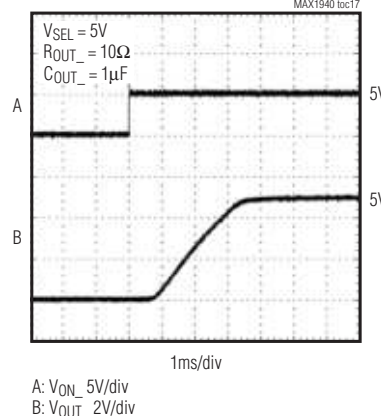
SWITCH TURN-ON TIME ( t_{ON} + t_{RISE} )
