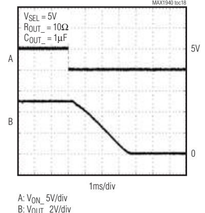
SWITCH TURN-ON TIME ( t_{ON} + t_{FALL} )
