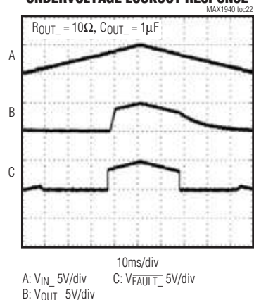
UNDERVOLTAGE LOCKOUT RESPONSE
