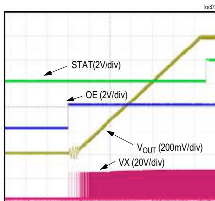
STARTUP RESPONSE
