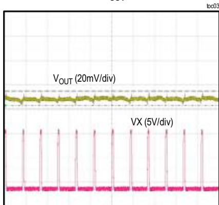
TYPICAL V_{OUT} RIPPLE
