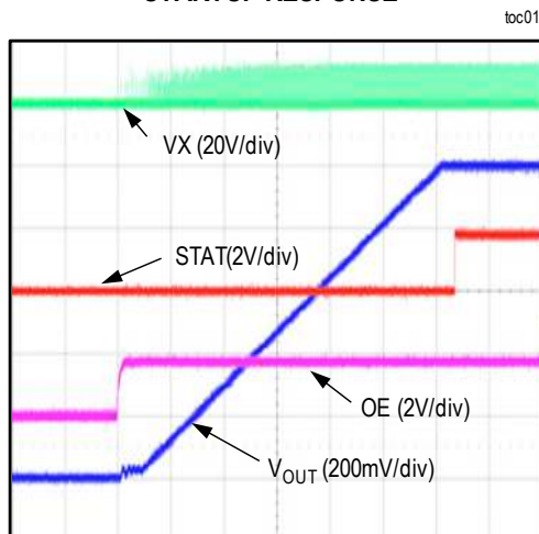
STARTUP RESPONSE
