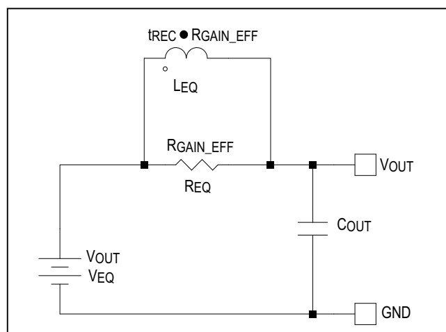
Figure 4. Averaged Small-Signal Equivalent Circuit of Regulator
