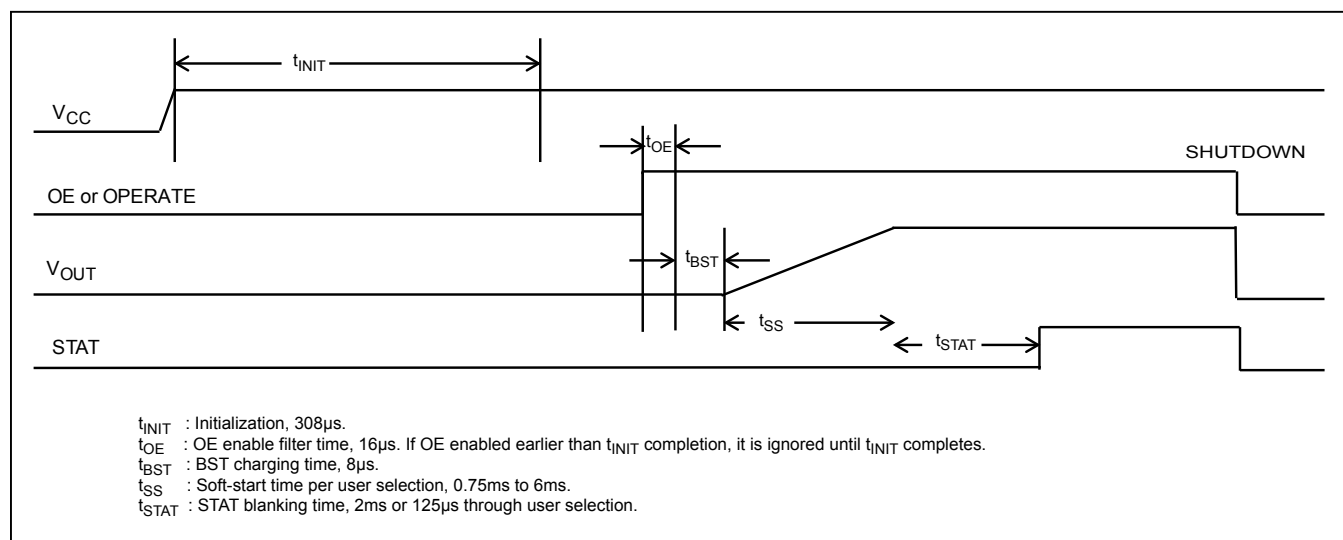
Figure 1. Startup Timing
