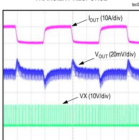
TRANSIENT RESPONSE
