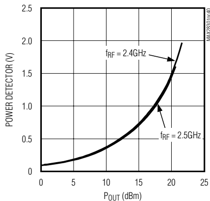
POWER DETECTOR OVER FREQUENCY
