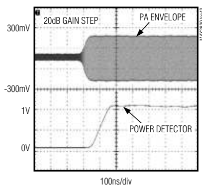
POWER-DETECTOR OUTPUT
