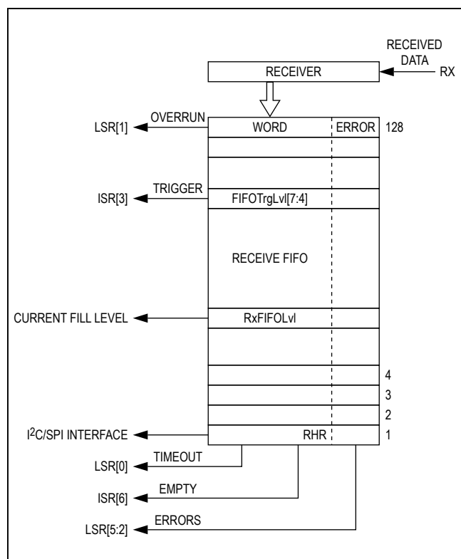
Figure 6. Receive FIFO
