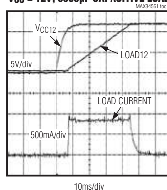
TURN-ON WAVEFORMS V CC = 12V, 3300μF CAPACITIVE LOAD
