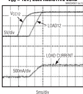
TURN-ON WAVEFORMS V CC = 12V, 20Ω RESISTIVE LOAD
