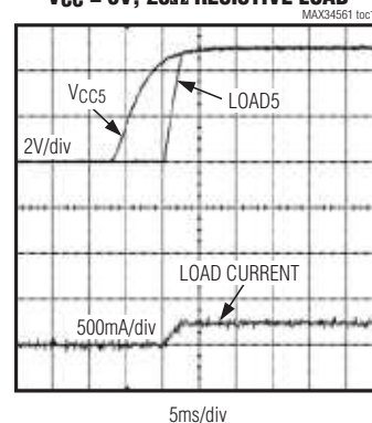
TURN-ON WAVEFORMS V CC = 5V, 20Ω RESISTIVE LOAD
