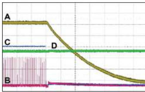
Shutdown with V_{CC} , Internal VREF
