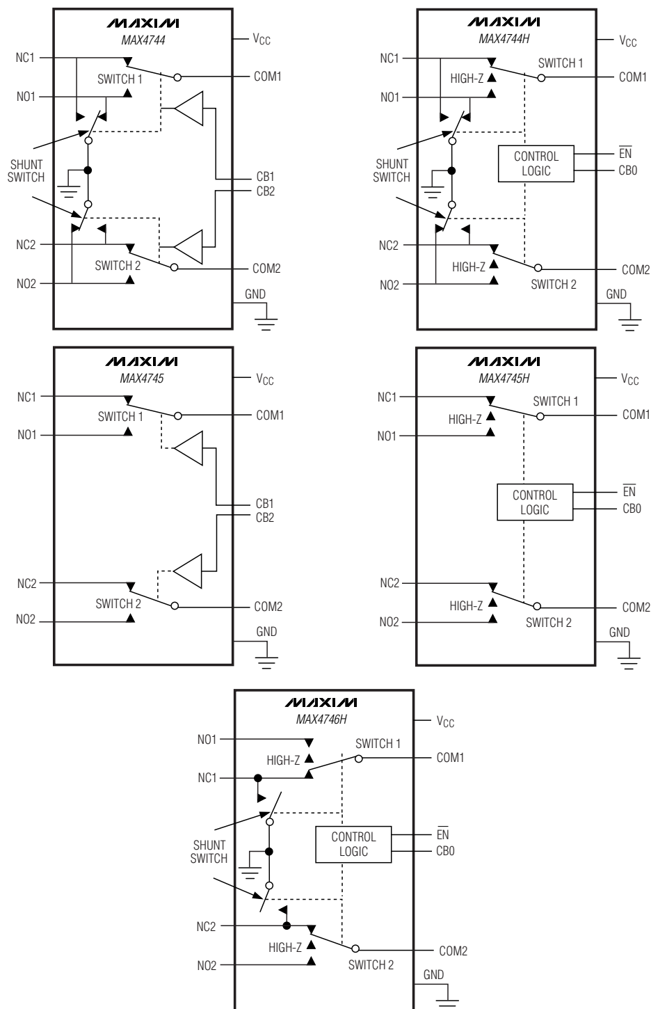
Figure 1. Functional Diagram
