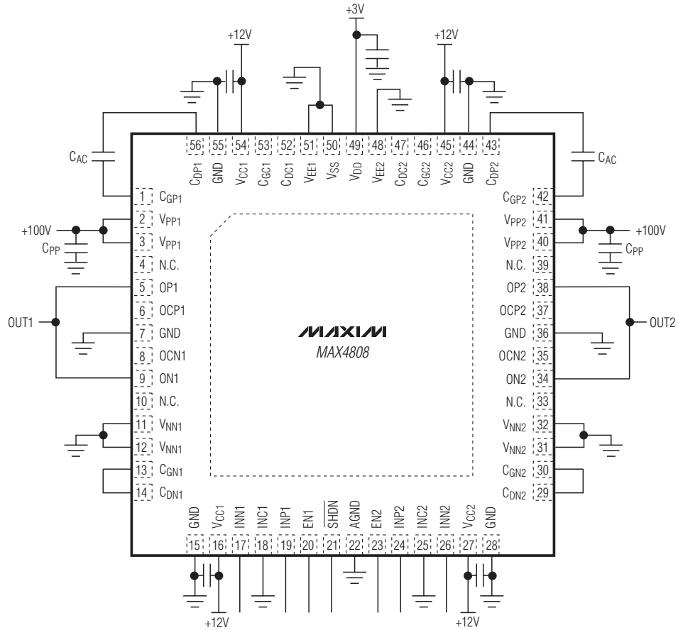
Figure 10. MAX4808: Dual Unipolar Pulsing, +100V, GND
