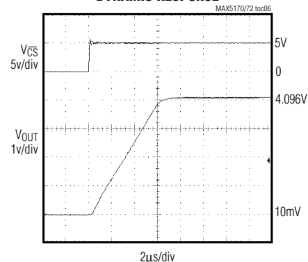
DYNAMIC RESPONSE
