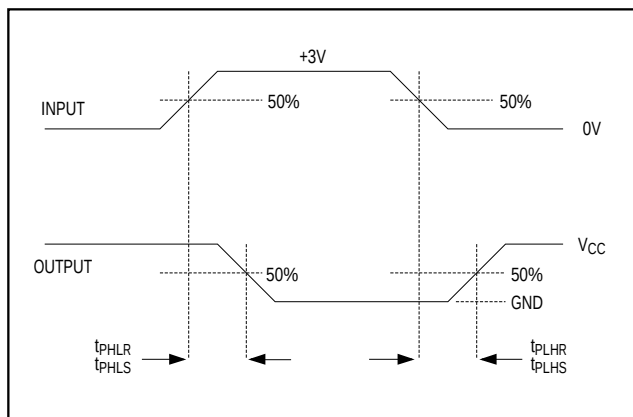
Figure 3. Receiver Propagation Delay Timing
