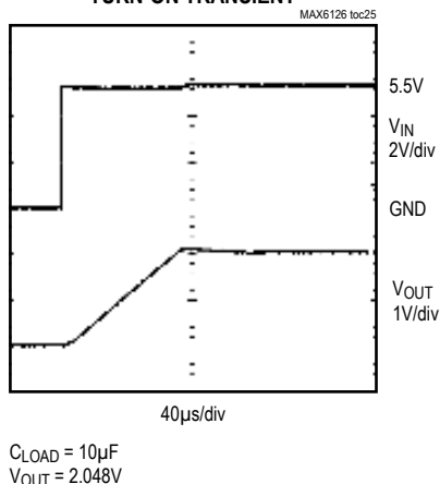
MAX6126_21 TURN-ON TRANSIENT
