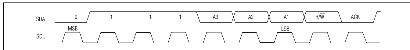
Figure 5. Slave Address
