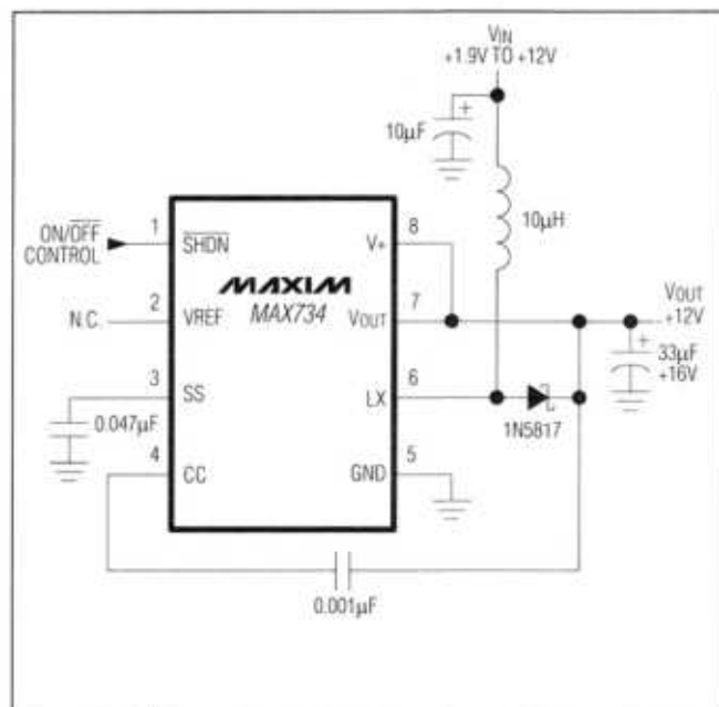
Figure 3: Bootstrap Operation
