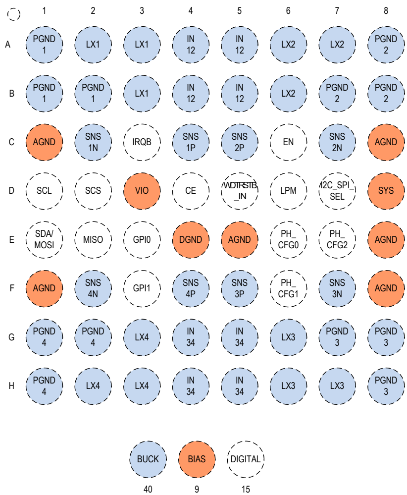
64 WLP (8 x 8 BUMP ARRAY, 0.4MM PITCH) *TOP VIEW = WAFER BACK-SIDE VIEW (BUMPS ARE NOT VIEWABLE)
