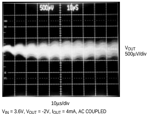
MAX843/MAX844 OUTPUT NOISE AND RIPPLE ( C_1 = C_2 = C_3 = 1\mu F , C_4 = 10\mu F )
