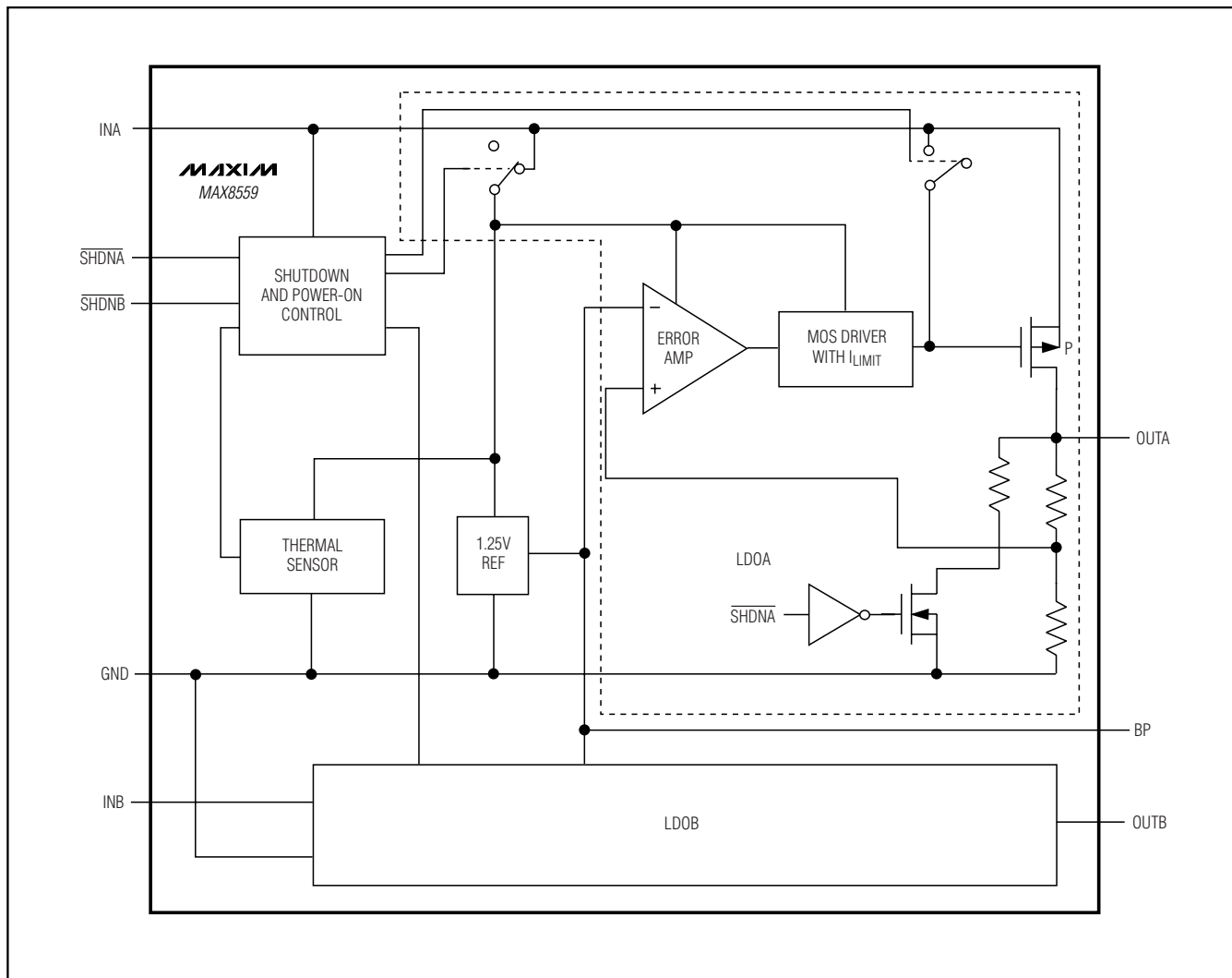
Functional Diagram
