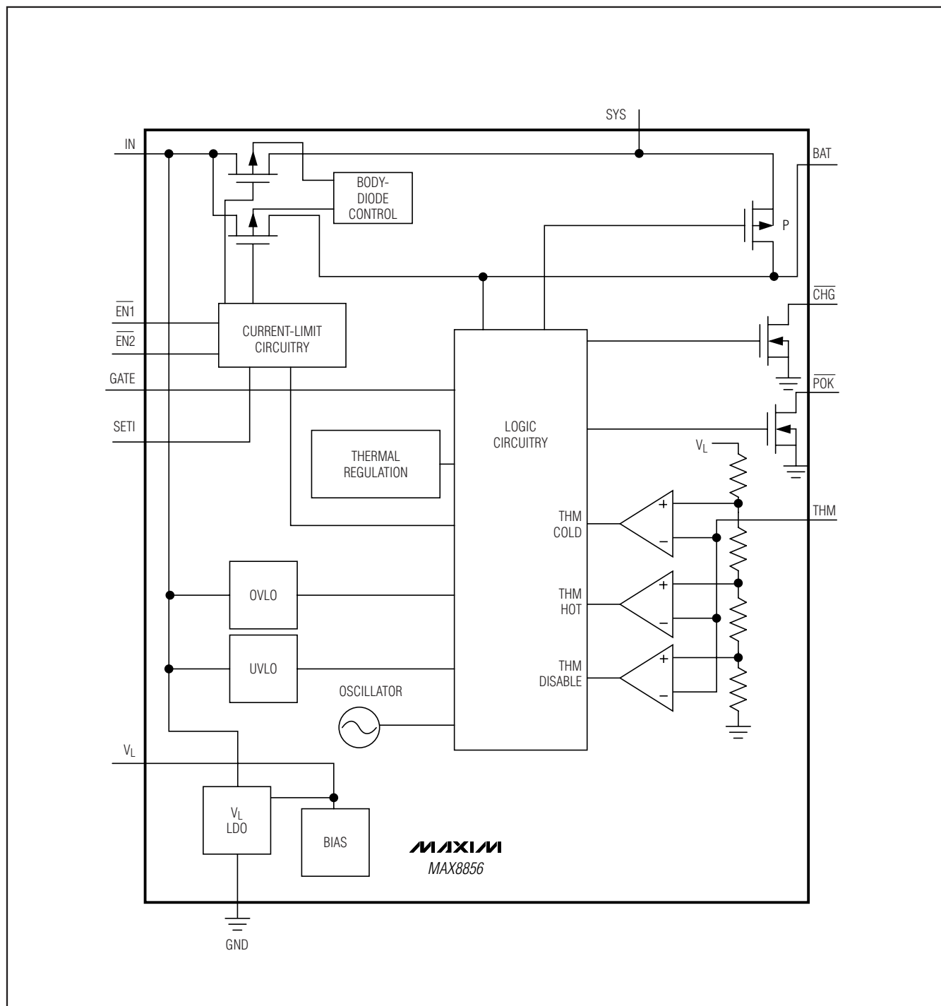
Figure 2. MAX8856 Block Diagram
