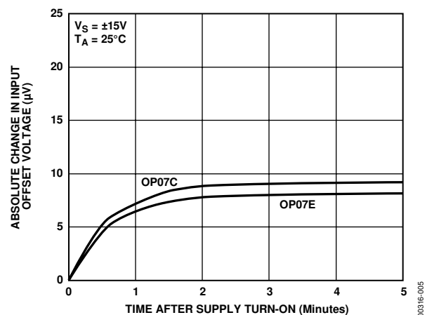
Figure 5. Warm-Up Drift
