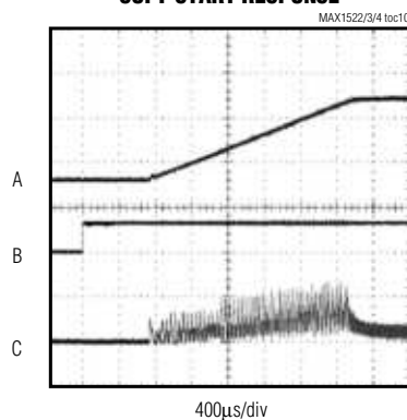
SOFT-START RESPONSE
