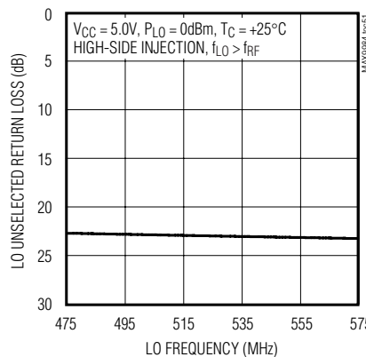
LO UNSELECTED RETURN LOSS vs. LO FREQUENCY (TUNED FOR 400MHz TO 500MHz RF FREQUENCY)
