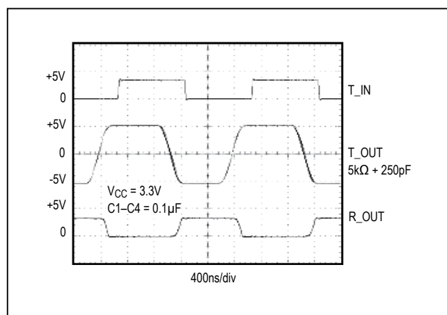
Figure 10. MAX3237E Loopback Test Result at 1000kbps (MBAUD = V_{\text{CC}} )
