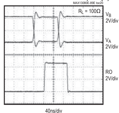
RECEIVER PROPAGATION DELAY (16Mbps)
