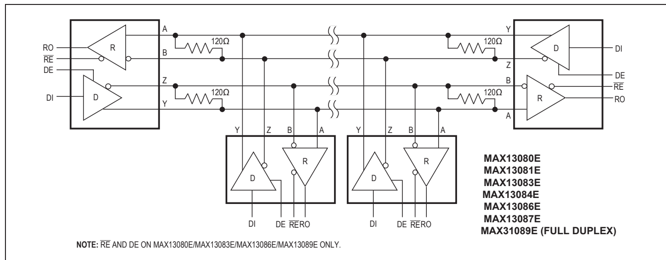
Figure 13. Typical Full-Duplex RS-485 Network
