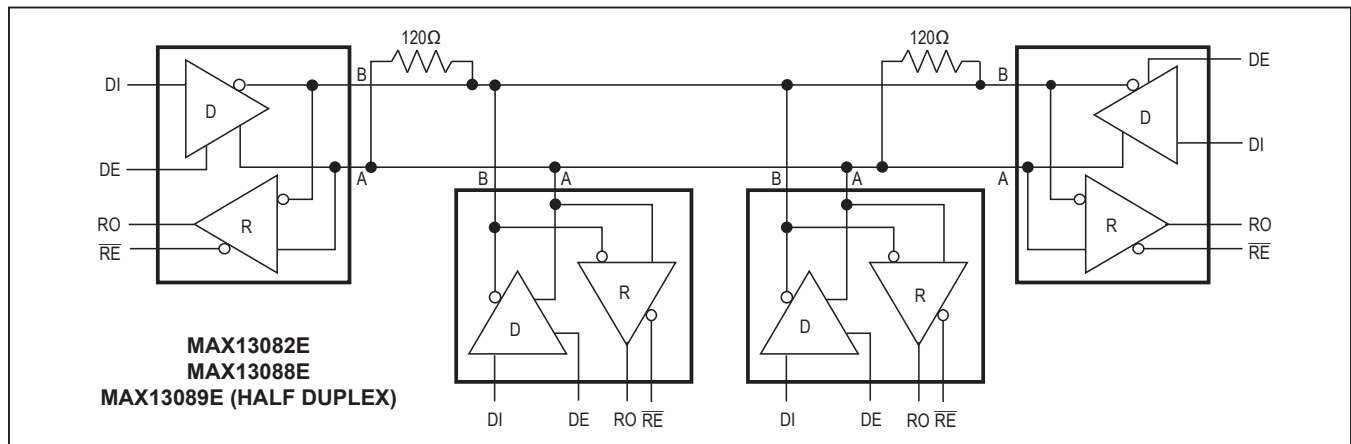
Figure 12. Typical Half-Duplex RS-485 Network
