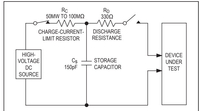
Figure 10c. IEC 61000-4-2 ESD Test Model
