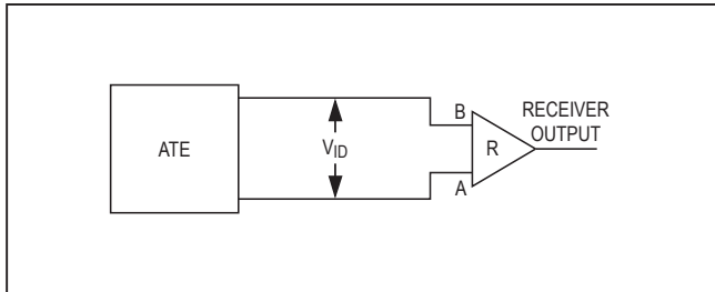
Figure 6. Receiver Propagation Delay Test Circuit
