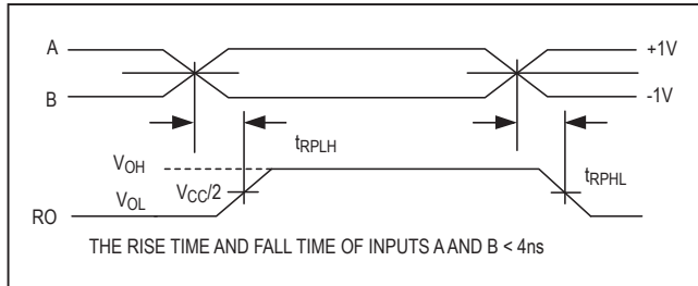
Figure 7. Receiver Propagation Delays
