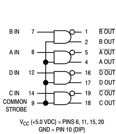
Figure 1. Logic Diagram
