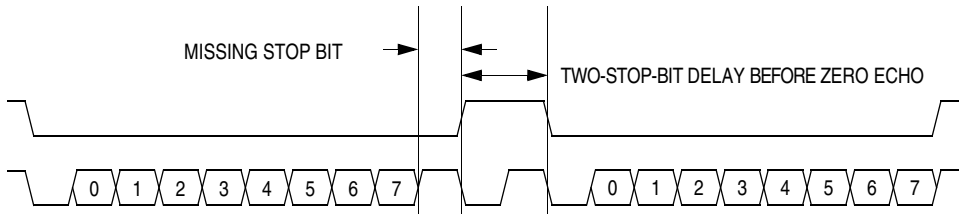
Figure 7-6. Break Transaction
