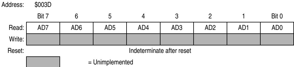
Figure 10-4. ADC Data Register (ADR)
