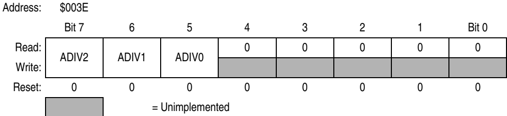
Figure 10-5. ADC Input Clock Register (ADICLK)
