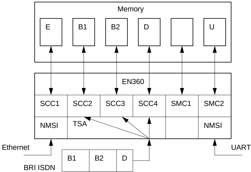
Figure 1-3. Internal Routing for Ethernet-to-BRI Bridge Using MC68EN360
