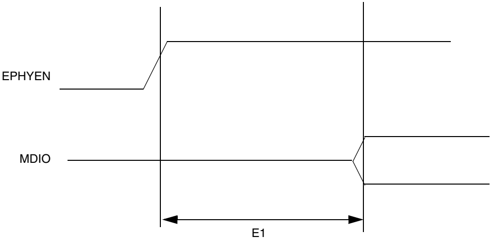
Figure 9. EPHY Timing
