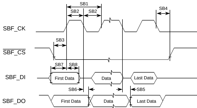
Figure 27. SBF Timing
