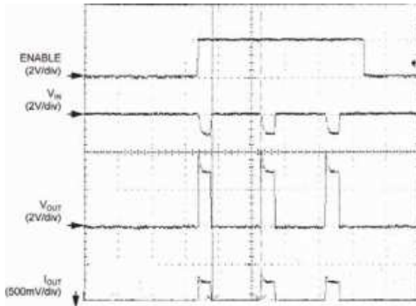
Figure 9. VUVLO Operation
