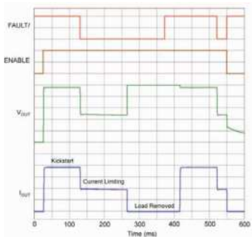
Figure 11. Kickstart™
