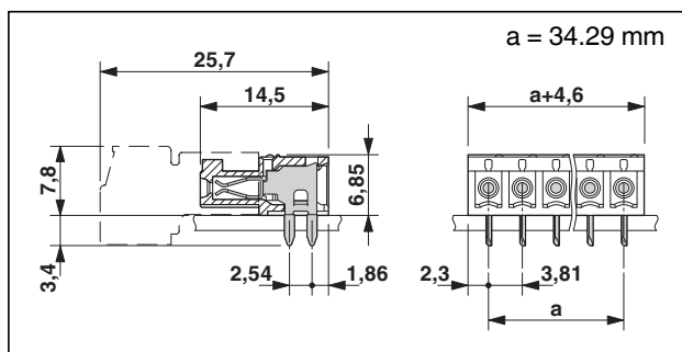
Figure 35 Dimensions IMC 1.5/10-G-3.81
